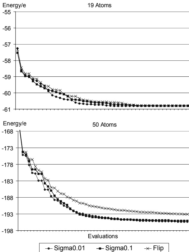
Figure 1: Evolution of MBF for instances with 19 and 50 atoms
